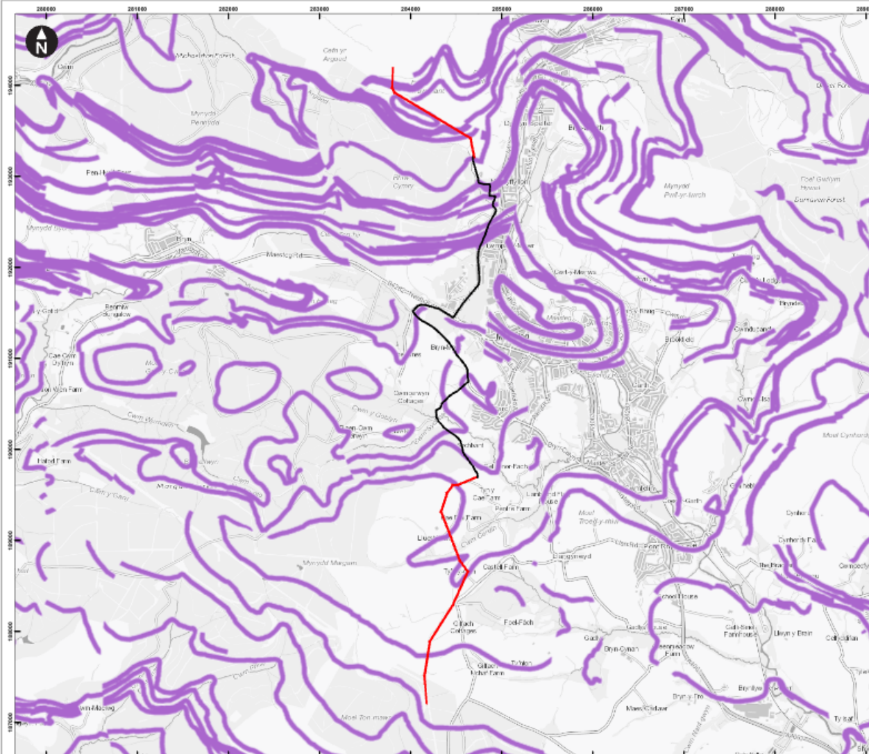
Figure 4B.4 MRA mapped coal outcrops
